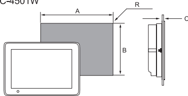
面板开孔尺寸: GC-4501W
